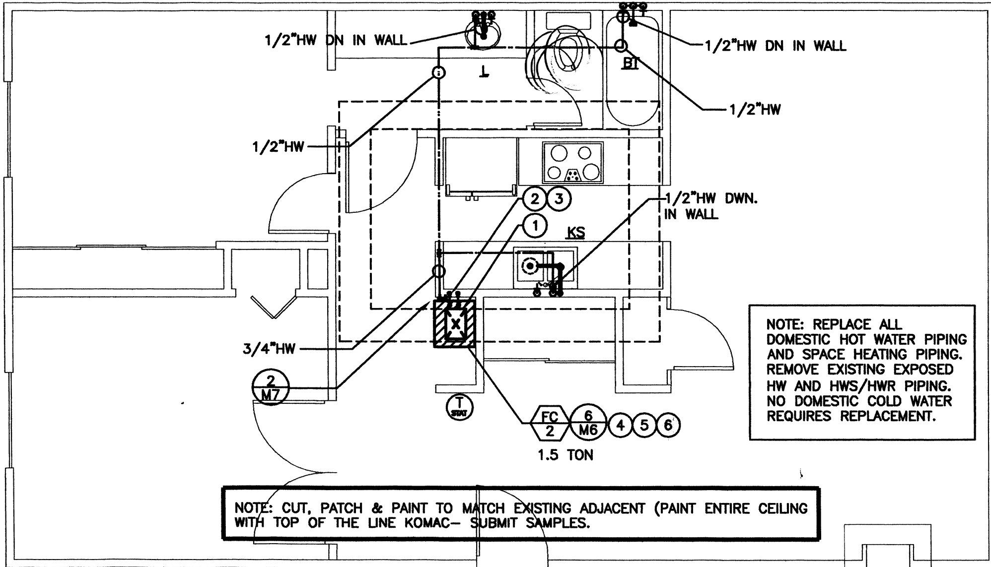
2 ONE BEDROOM / DEN PLAN M-6 SCALE: 1/4" - 1'-0"
