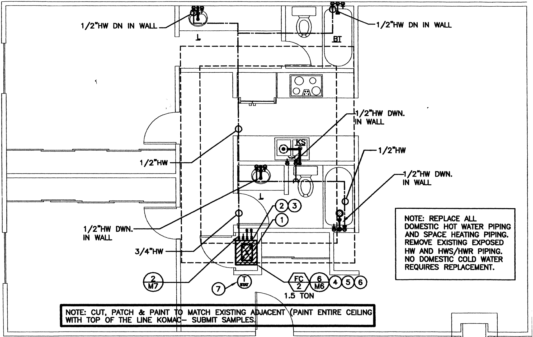
3 TWO BEDROOM PLAN M-6 SCALE: 1/4" - 1'-0"
